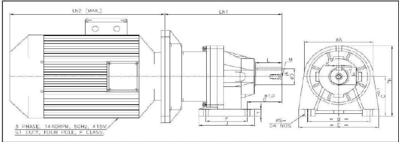
DIMENSIONS OF GEARED MOTOR FOOT MOUNTED
