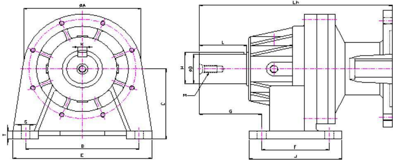
DIMENSIONS OF FOOT MOUNTED HOLLOW INPUT
