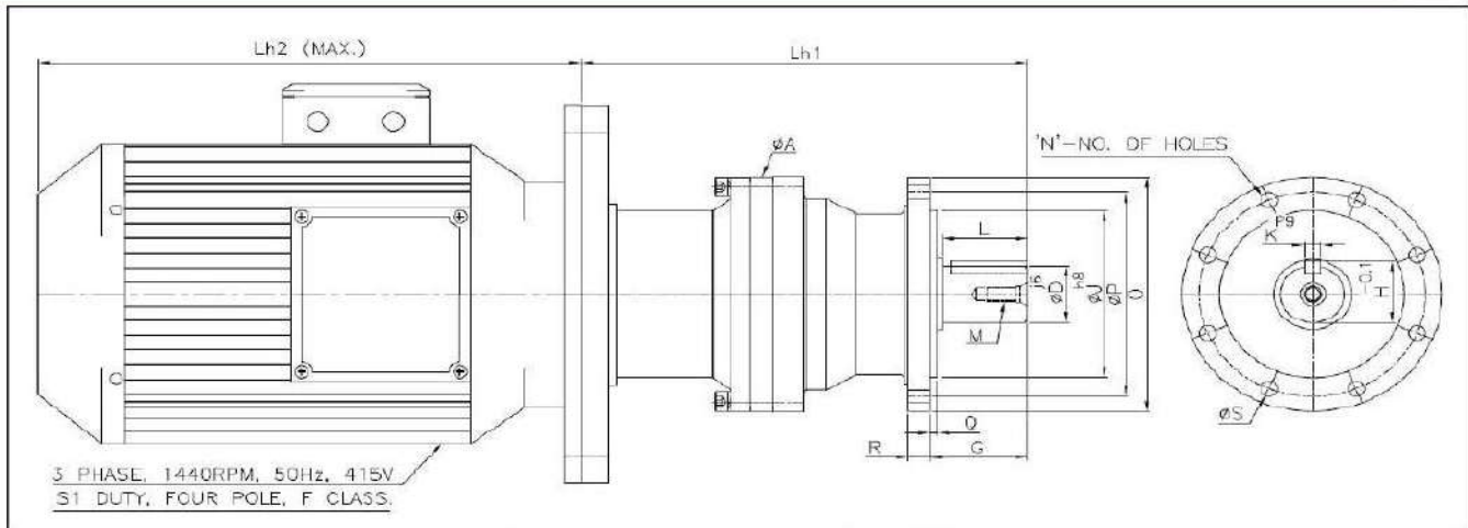
DIMENSIONS OF GEARED MOTOR FLANGE MOUNTED
