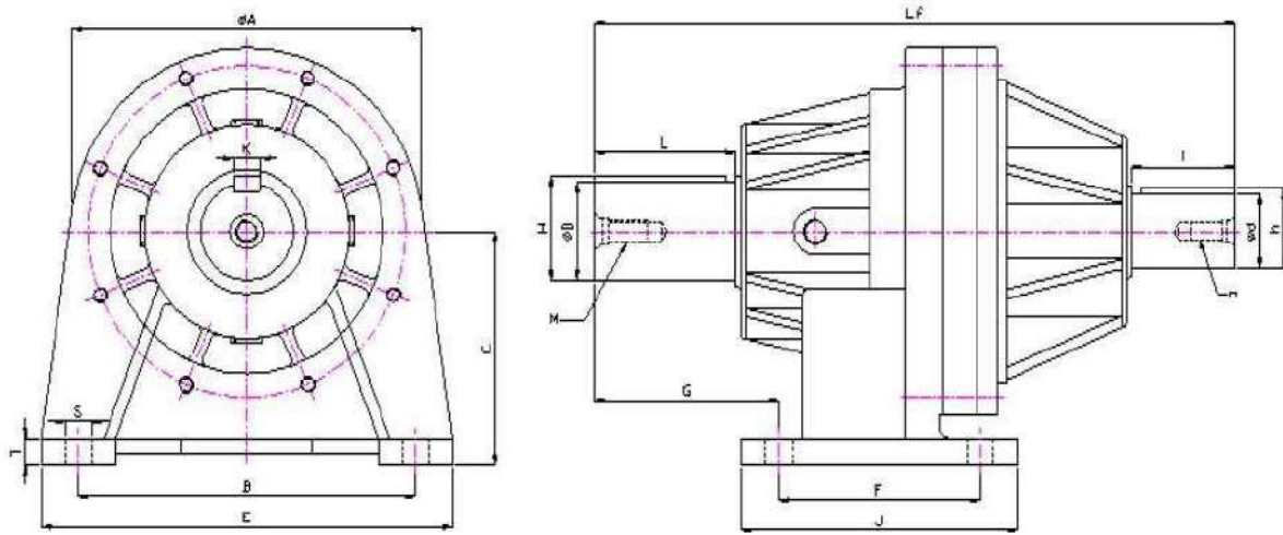
DIMENSIONS OF FOOT MOUNTED FREE INPUT
